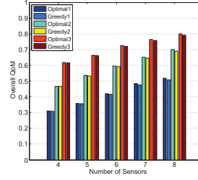
Fig. 3. Greedy vs optimal
