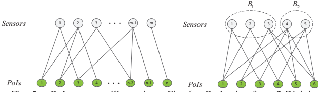
Fig. 5. PoI coverage illustration Fig. 6. Reduction from 2-Disjoint set cover problem
