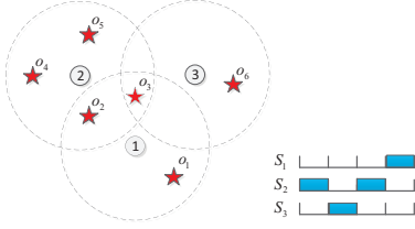
Fig. 2. An example of scheduling
