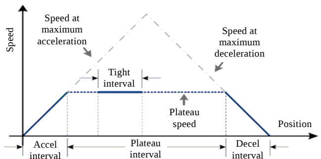
Fig.7 Different stages of speed adjust of MDC
