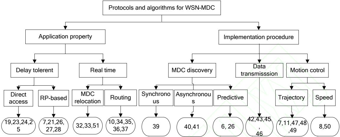
Fig.8 Protocols and algorithms for WSN-MDC: A taxonomy
